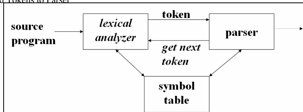
Fig 1: Lexical Analyzer
